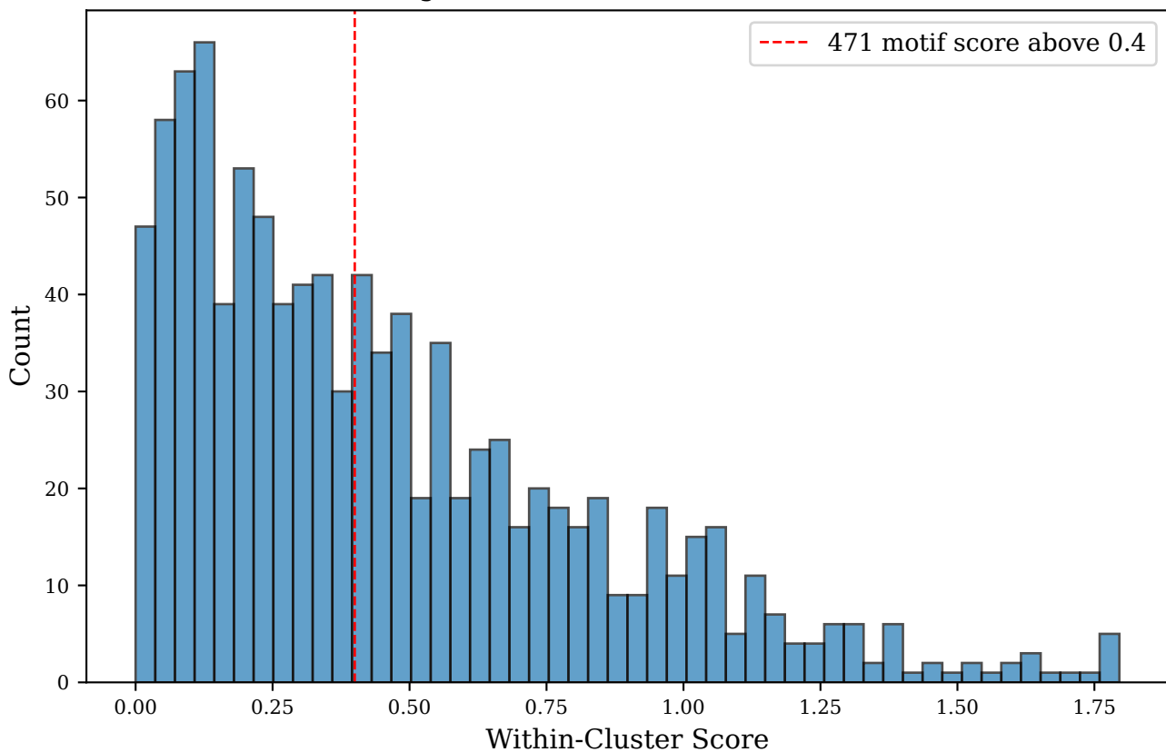
Distribution of All Motif Scores (50 seeds, 1000 motifs total) \sigma=(0.02, 0.4) , \text{vol}=(0.07, 0.9)
